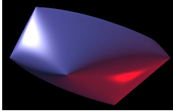
Figure 3.1: A spectrahedron.
